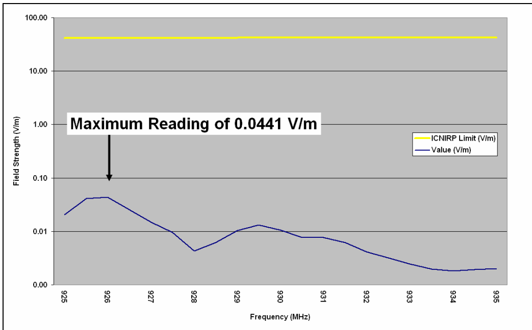
Figure 9 – Wave Spectrum Scan Graph (900MHz)
