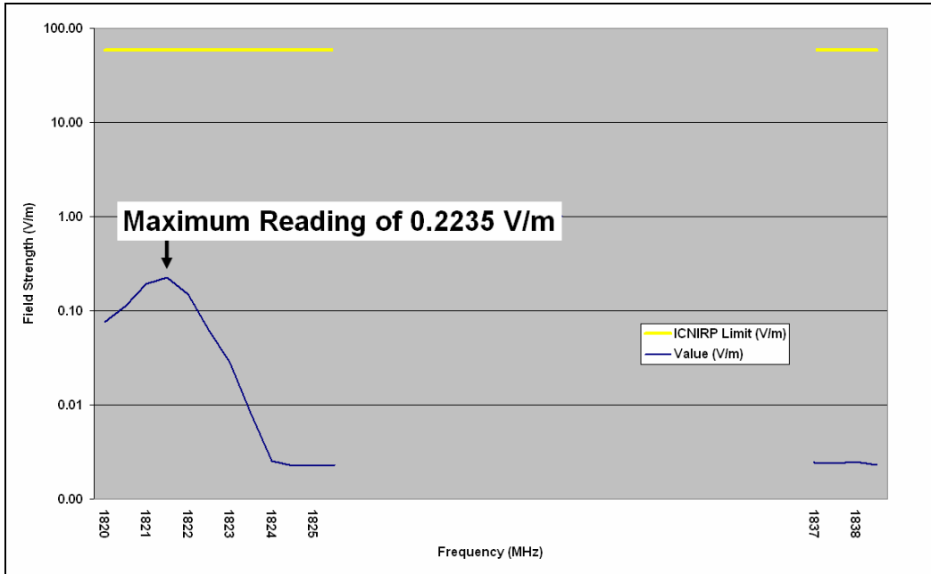
Figure 6 – Airtel Spectrum Scan Graph (1800MHz)
