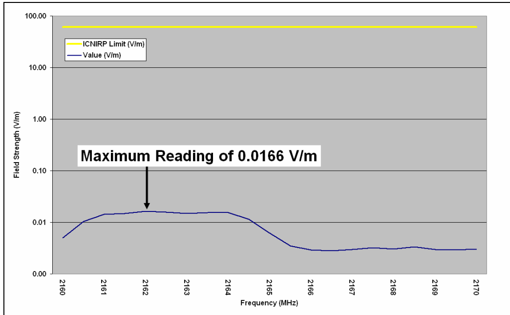
Figure 7 - Airtel Spectrum Scan Graph (UMTS)
