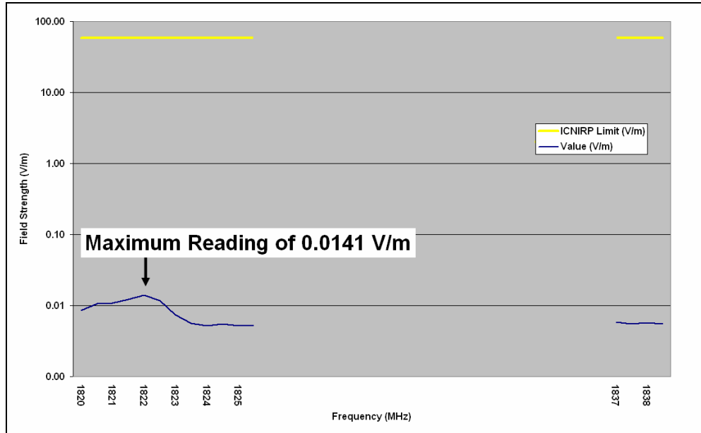
Figure 6 – Airtel Spectrum Scan Graph (1800MHz)
