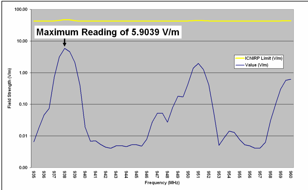
Figure 5 – C&W Spectrum Scan Graph (900MHz)
