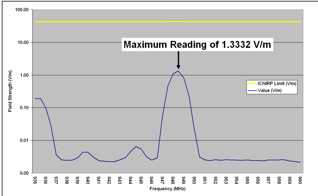
Figure 6 – C&W Spectrum Scan Graph (900MHz)
