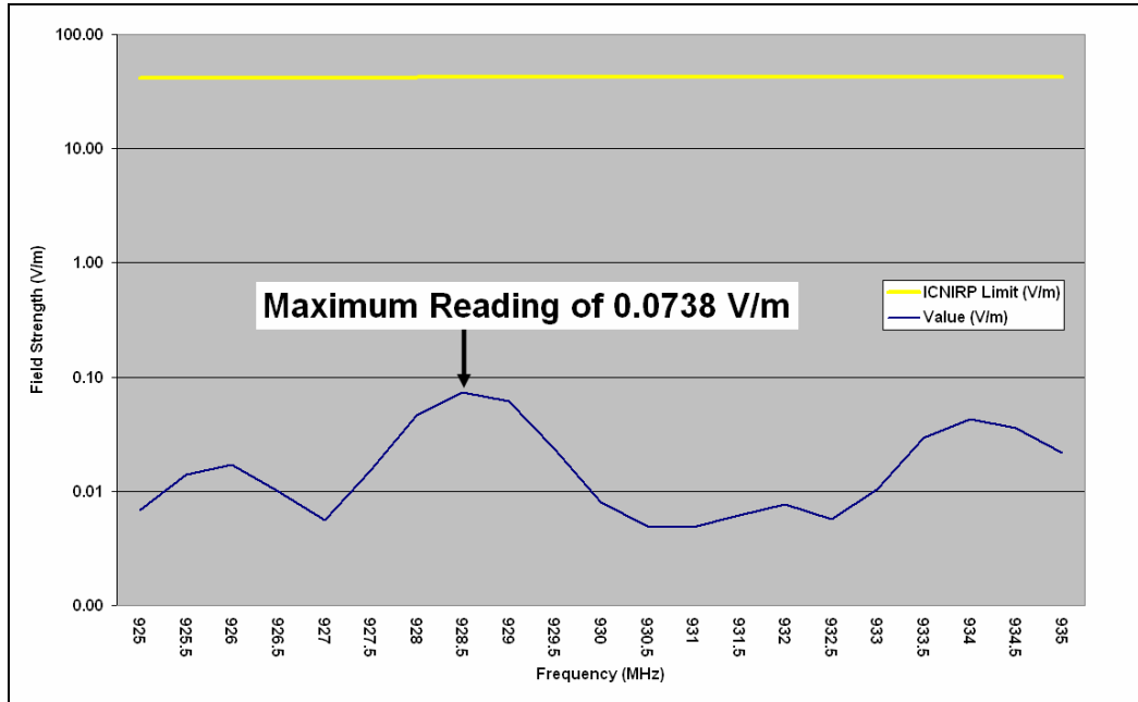
Figure 10 - Wave Spectrum Scan Graph (900MHz)
