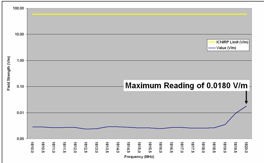
Figure 11 - Wave Spectrum Scan Graph (1800MHz)
