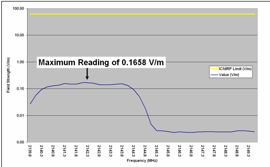
Figure 9 - Wave Spectrum Scan Graph (UMTS)
