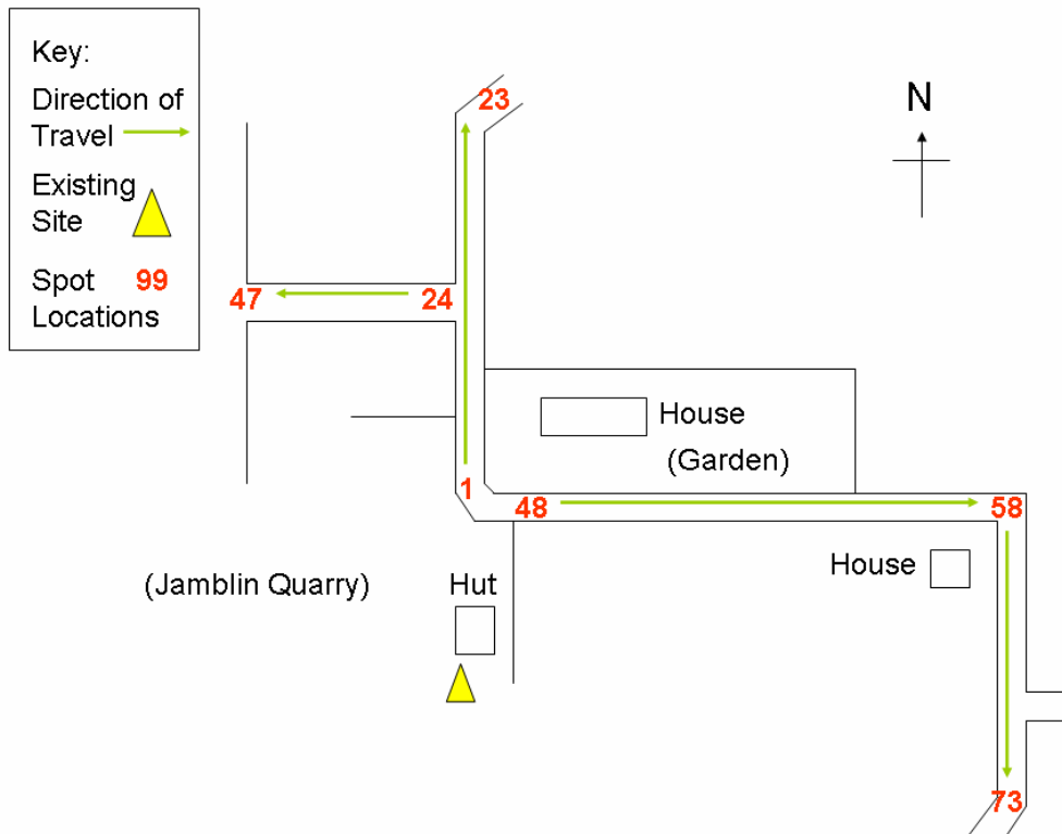
Figure 7 – Survey Area with Spot Measurement Markers
