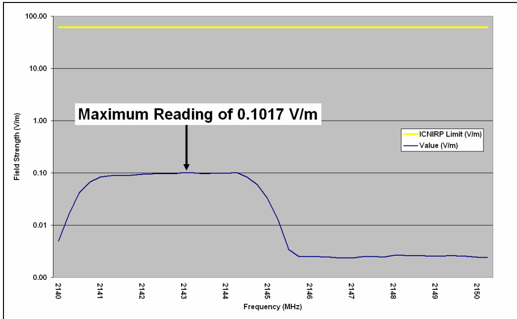
Figure 7 - Wave Spectrum Scan Graph (UMTS)
