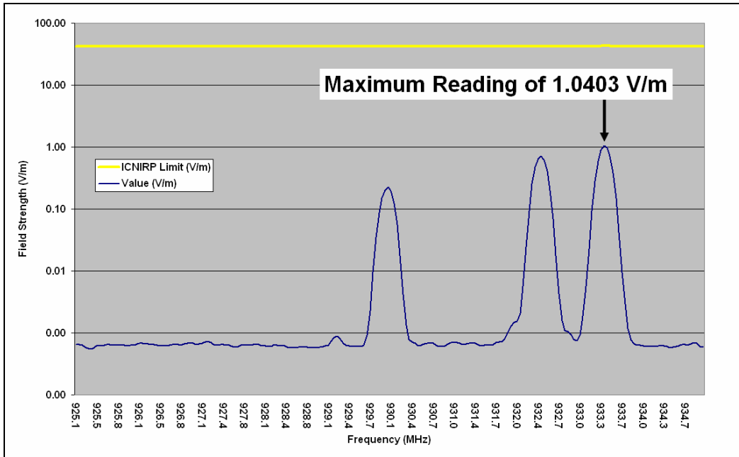
Figure 7 – Wave Spectrum Scan Graph (900MHz)
