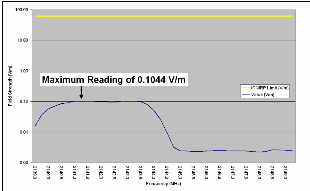
Figure 8 - Wave Spectrum Scan Graph (UMTS)
