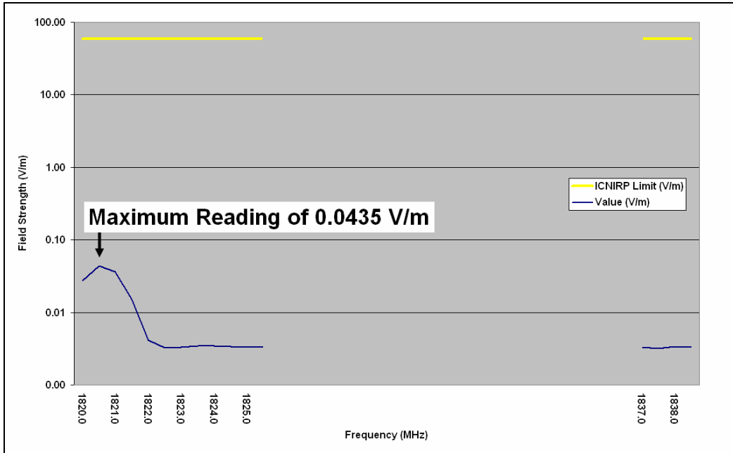
Figure 9 – Airtel Spectrum Scan Graph (1800MHz)
