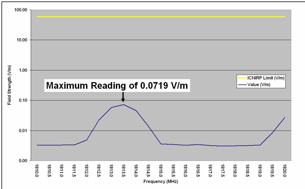
Figure 8 - Wave Spectrum Scan Graph (1800MHz)
