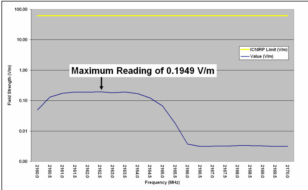
Figure 10 - Airtel Spectrum Scan Graph (UMTS)
