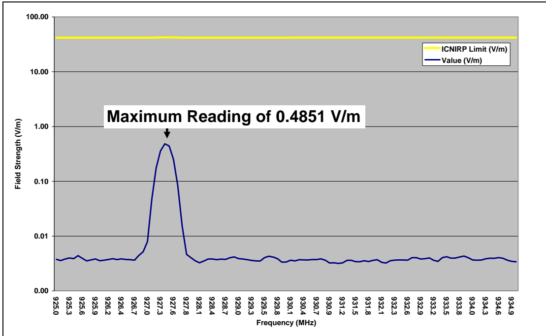
Figure 7 – Wave Telecom Spectrum Scan Graph (900MHz)
