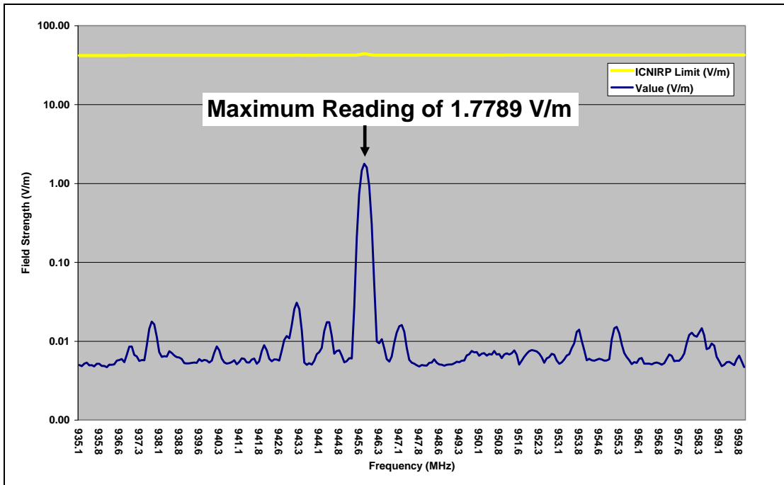
Figure 9 – C&W Spectrum Scan Graph (900MHz)
